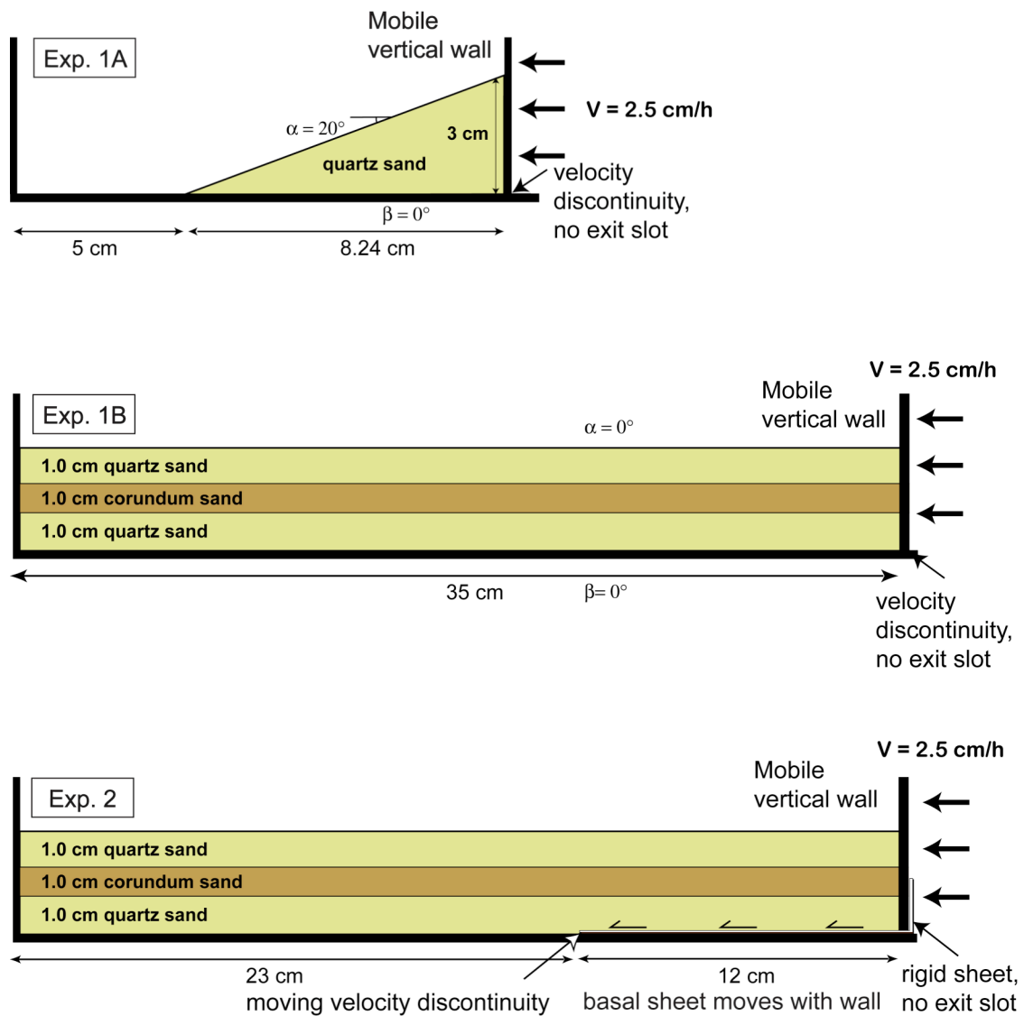
Fig. 1. Experimental set-ups used in analogue model comparisons
